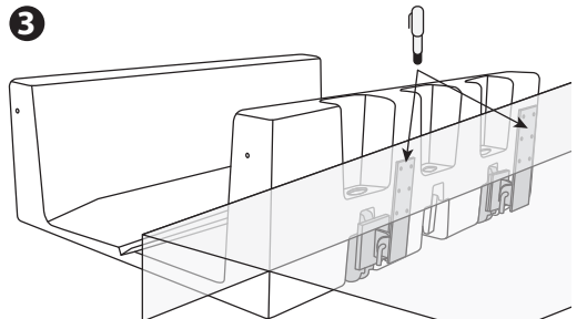
See-through-view of Floating Dock
