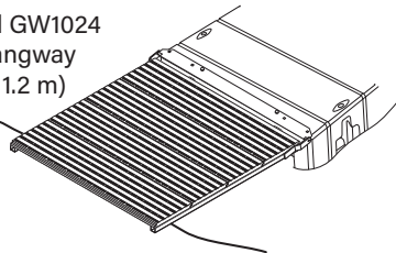
Assembled GW1028 4' x 8' Gangway (1.2 m x 2.4 m)
