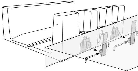
See-throught-view of Floating Dock
