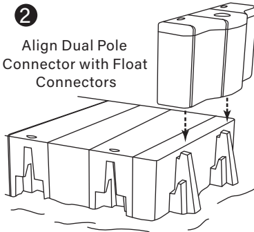
Float Connector
